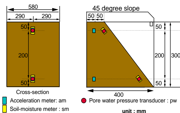
Figure.2.29 Model shapes and locations of measurement devices
