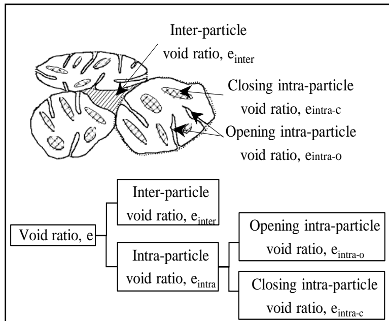
Figure.2.21 Schematic diagram of void ratio in volcanic soil (revision of Nakata and Miura 2007)
