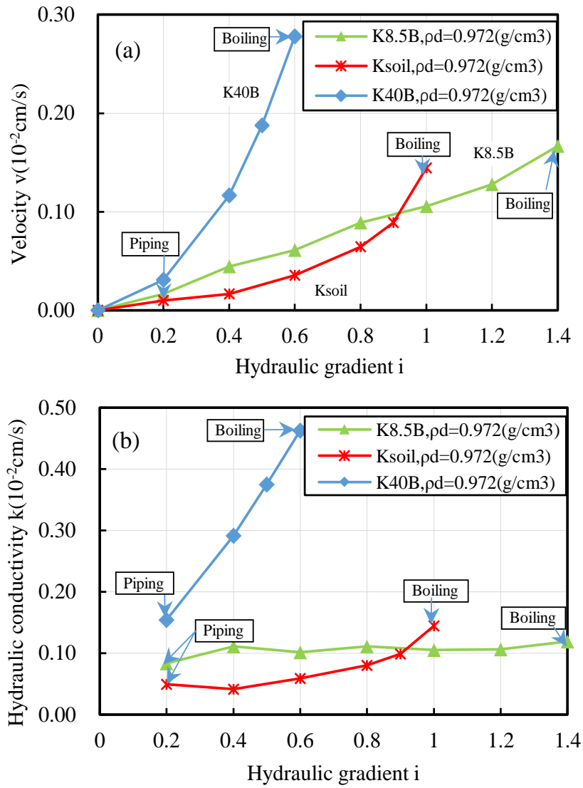
Figure.5.18 Test results of K_{\text{soil}} , K_{8.5B} and K_{40B} : (a) velocity, (b) hydraulic conductivity.
