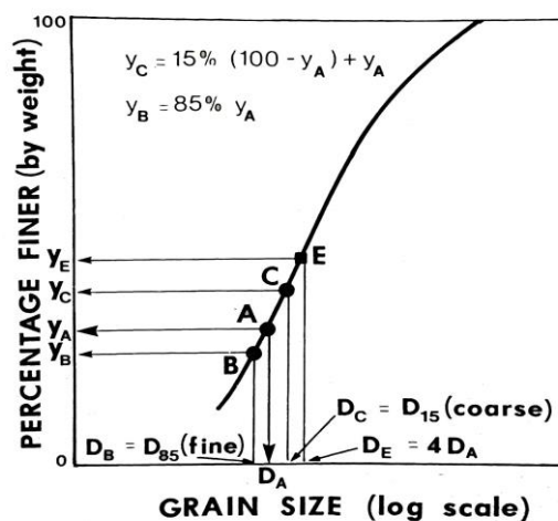
Figure.2.7 Illustration of relationship between the criteria about suffusion by Chapuis (1992)
