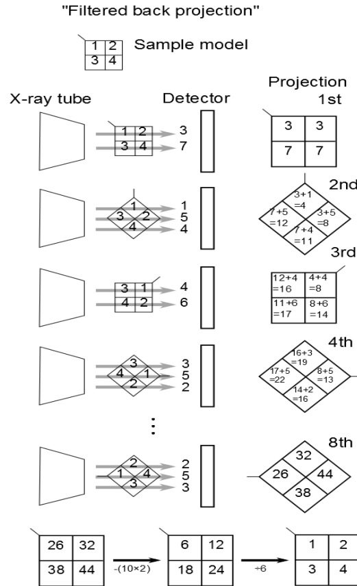
Figure.4.8 Principle of image acquisition and reconstruction
