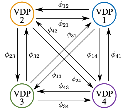
Fig.1: VDP coupling(All coupling)
