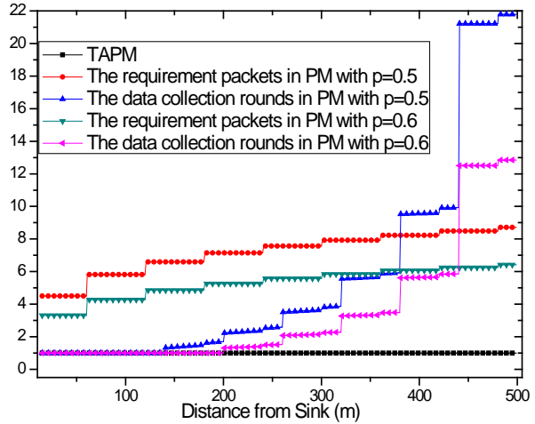
Fig. 14 The traceback time (the data collection rounds need to reconstruct the attack path ) with success probability is 0.9
