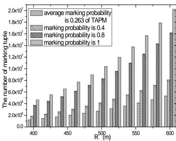
Fig. 23 The total marking tuples under different R
