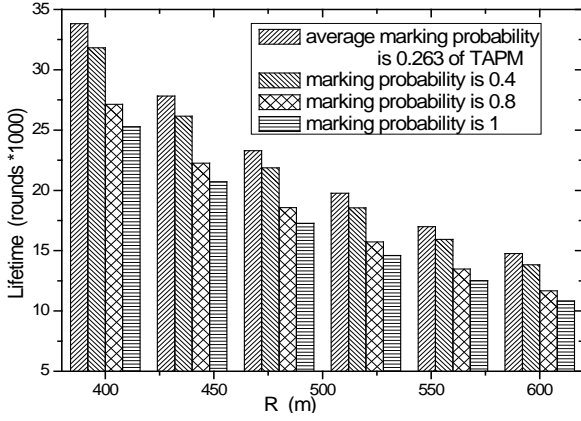
Fig. 33 The lifetime under different R with the length of marking tuple is 0.3 of the length of data packet
