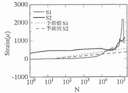
(c) No.6 V_{max}=35.0\text{kN} p_w=0.40\%
