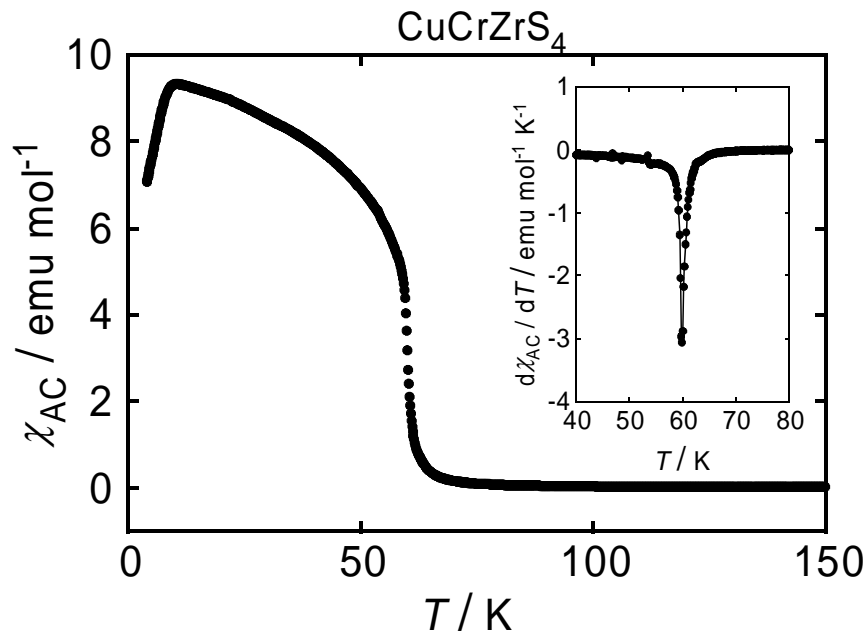
Figure 7. Temperature dependence of the ac magnetic susceptibility \chi_{AC} for CuCrZrS 4 as a function of temperature. The demagnetizing field corrections have been made. The inset shows the temperature derivative of \chi_{AC} , which indicates the T_c at sharp negative peak.
