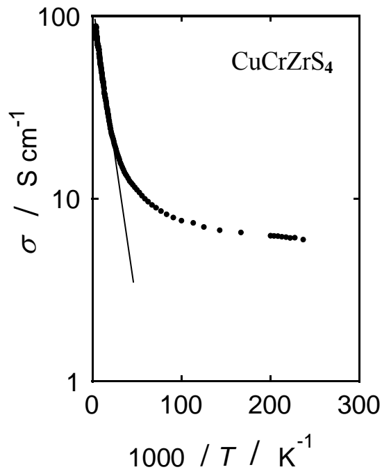
Figure 4. Temperature dependence of electrical conductivity \sigma=1/\rho for a sintered \text{CuCrZrS}_4 specimen. The straight line indicates the result calculated for activation energy model for conduction.
