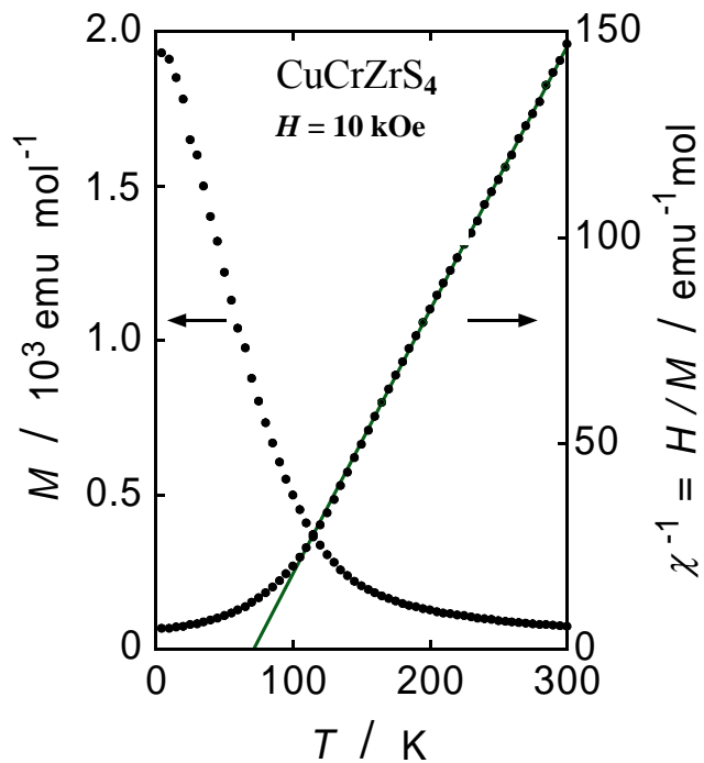
Figure 8. Temperature dependence of magnetization M and the inverse magnetic susceptibility \chi^{-1} = (M/H)^{-1} for CuCrZrS 4 in a constant field of 10.00 kOe. The straight line is the Curie-Weiss law.
