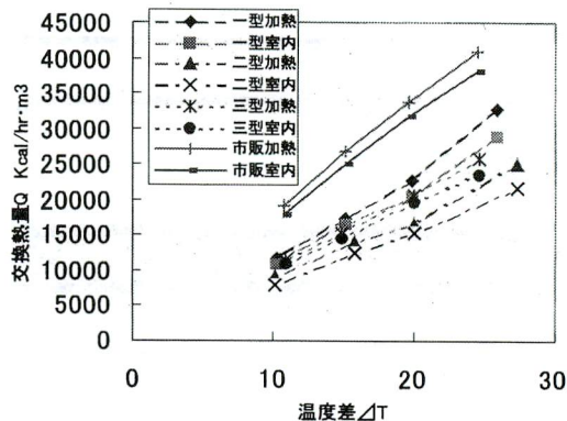
Fig.19 Characteristic of Exchanged Heat per Unit volume
