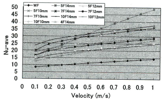
Fig.16 Average Nusselt Number
