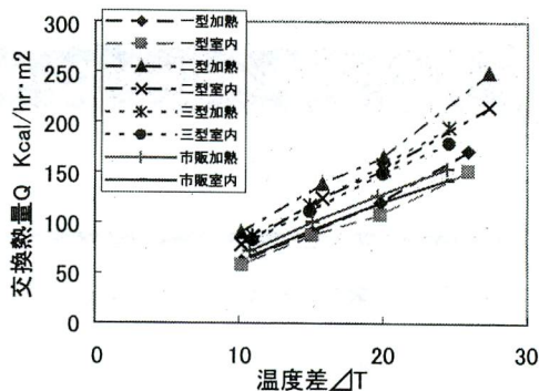
Fig.20 Characteristic of Exchanged Heat per Unit Area
