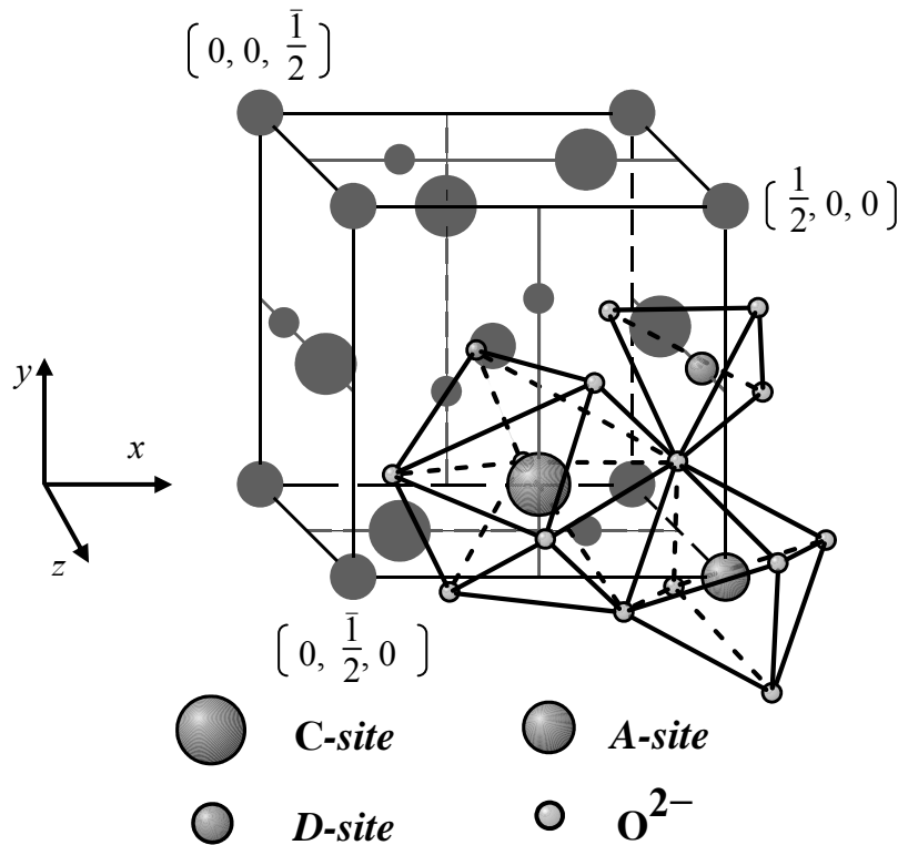
Figure 1. A skeleton drawing of an eighth of unit cell of garnet-type structure \{Y_{1-x}Gd_x\}_3Fe_5O_{12} with the dodecahedral \{C\text{-site: } Y \text{ or } Gd\} , octahedral [ A -site: Fe], and tetrahedral ( D -site: Fe) sites, emphasizing the C -, A - and D -sites. Unit cell of garnet-type structure has the space group Ia\bar{3}d (No. 230, O_h^{10} ).
