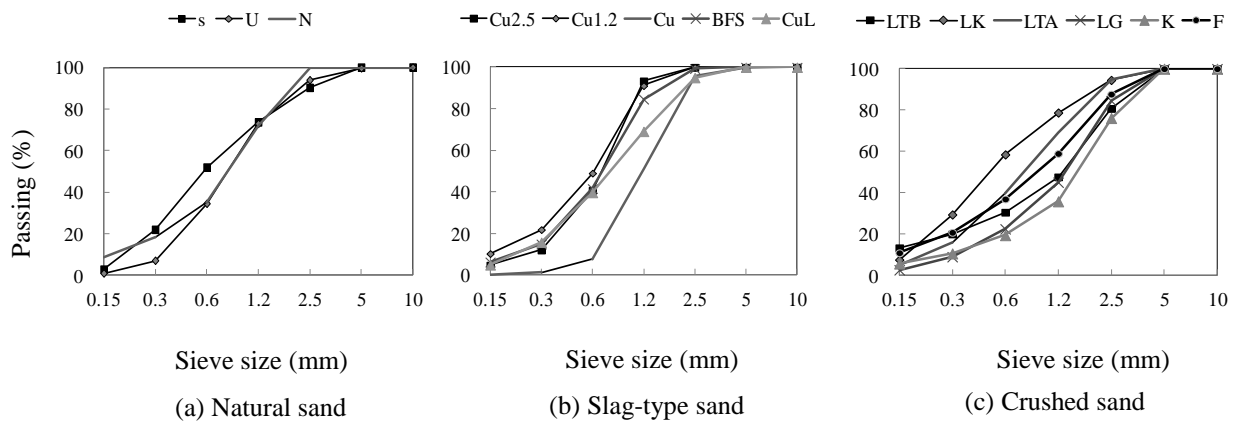
Fig. 1 Particle size distribution of fine aggregate used in mortar specimens.
