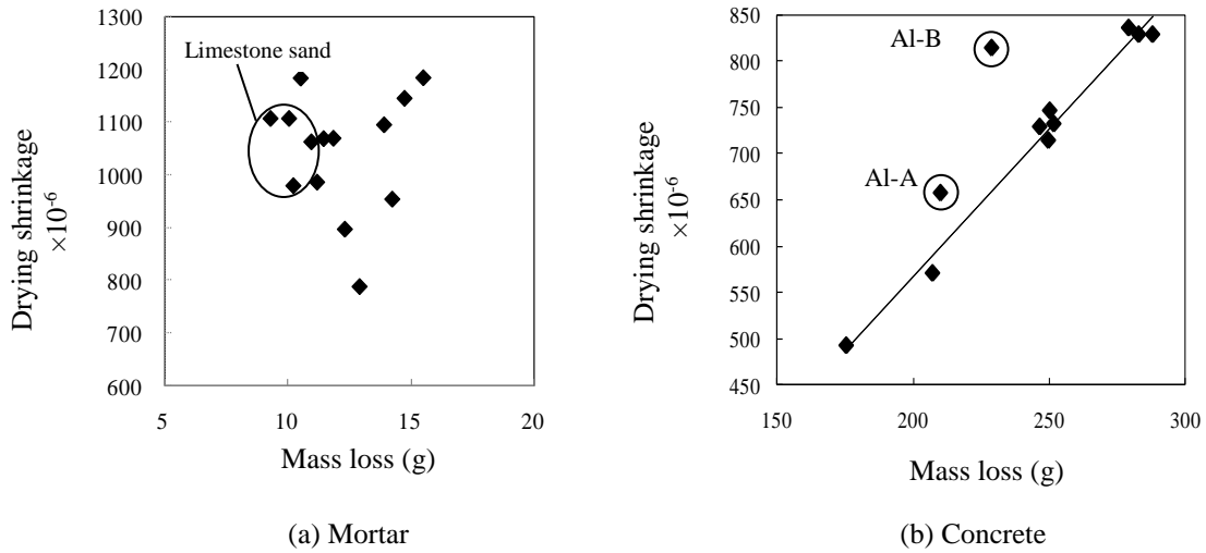
Fig. 6 Correlation between drying shrinkage and water mass loss.
