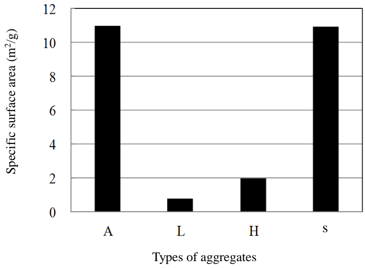
Fig. 10 Specific surface area results of aggregates.
