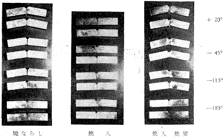
炭素鋼 No. 2 C. 0.28%
