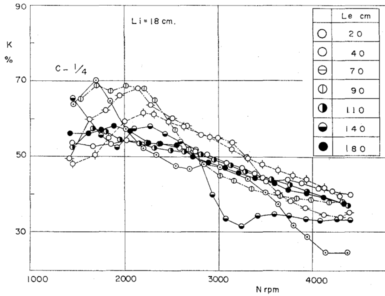
図-18 排気管効果 (E-50, C-1/4)
