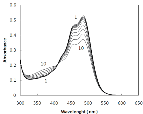
Fig. 5 Photoreaction of spR at 20^{\circ}\text{C} . spR (at 20^{\circ}\text{C} ; curve 1) was irradiated with 450 nm light for a total period of 1, 2, 4, 8, 16, 32, 64, 128 and 256 min (curve 2 – 10, respectively).
