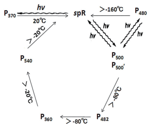
Fig. 6 Photocycle of pR
