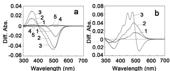
Fig. 4 Thermal reaction of PSS 450 from -80 to 10^{\circ}\text{C} . Panel a: Curve 1-5 indicate the difference spectral changes before and after each stepwise warming of PSS 450 from -80^{\circ}\text{C} to -60 , -50 , -40 , -30 , -20^{\circ}\text{C} , respectively. Panel b: Curve 1-3 indicate the difference spectral changes before and after each stepwise warming of PSS 450 from -80^{\circ}\text{C} to -10 , 0 , 10^{\circ}\text{C} , respectively. Each time immediately after warming to predetermined temperature, the mixture was cooled down to -80^{\circ}\text{C} to measure the absorption spectra.
