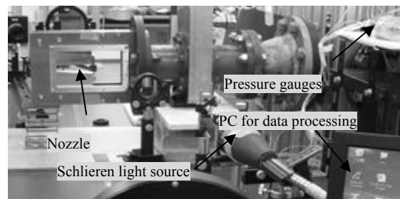
Fig. 1 Experimental setup
