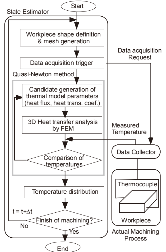
Fig.7 Configuration of thermal state estimation system (5)
