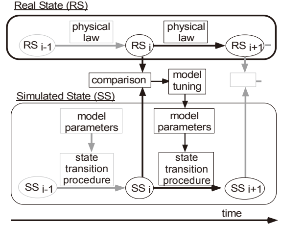
Fig.6 Adaptive estimation procedure
