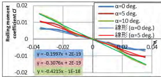
Fig. 3.1. C_l vs. \dot{p} .
