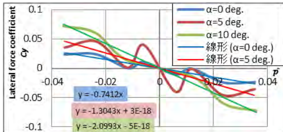
Fig. 3.3. C_y vs. \dot{p} .
