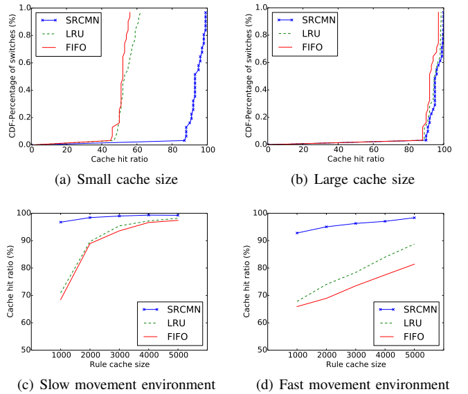
Fig. 5. Evaluation results outperform the comparison algorithm in both micro benchmark and large scale simulations.
