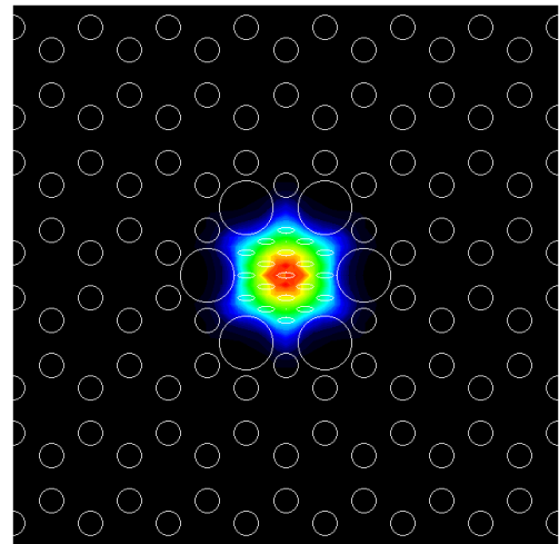
Fig. 7. Guided modes of a double single-polarization band PBG fiber shown in Fig. 6. (a) Effective index as function of normalized frequency for the x -polarized ( HE_{11}^x ) and y -polarized ( HE_{11}^y ) fundamental modes, which correspond to the blue-colored solid and red-colored dashed curves, respectively. (b) Mode field distribution for the HE_{11}^y mode at \Lambda/\lambda = 0.65 . (c) Mode field distribution for the HE_{11}^x mode at \Lambda/\lambda = 0.85 .
