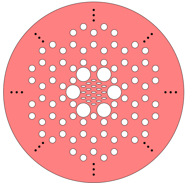
Fig. 6. Double single-polarization band PBG fiber.
